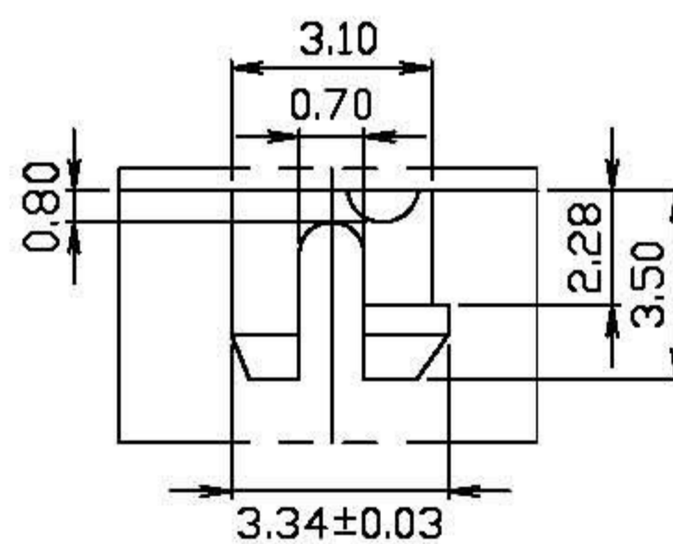
DETAIL X
