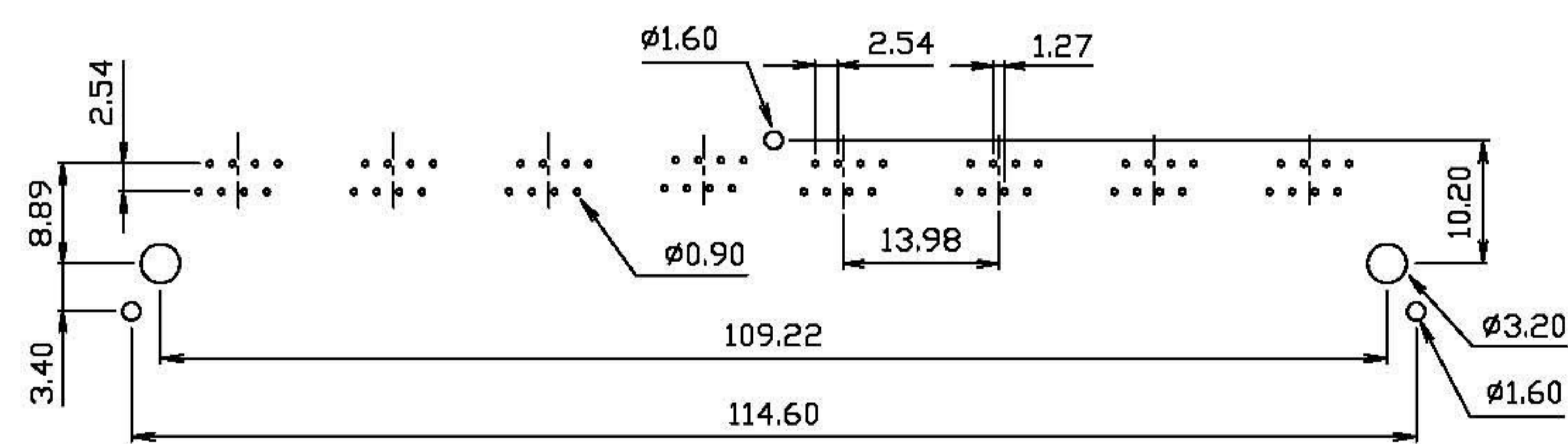
PC Board Layout
