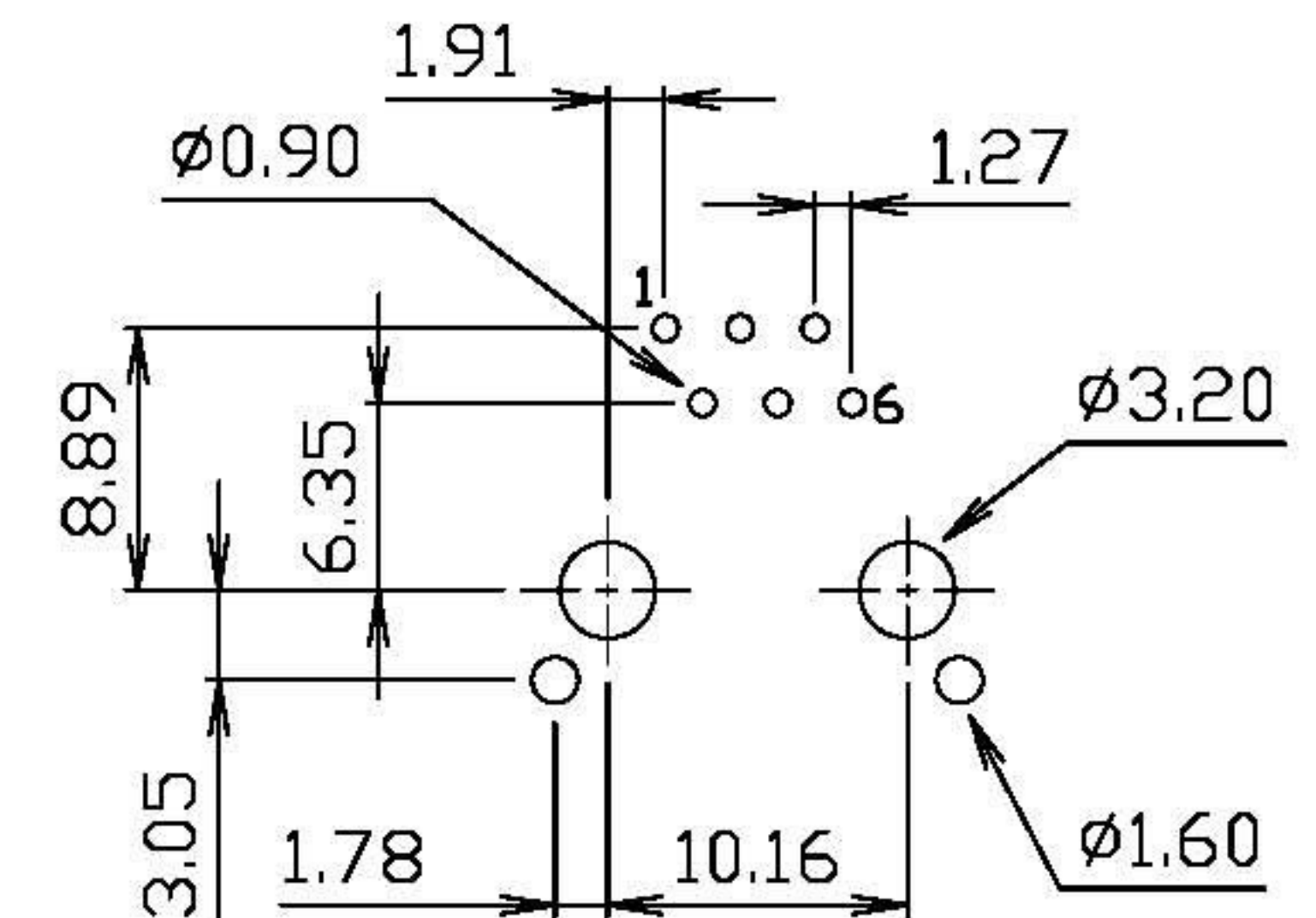
PC Board Layout Ref.
