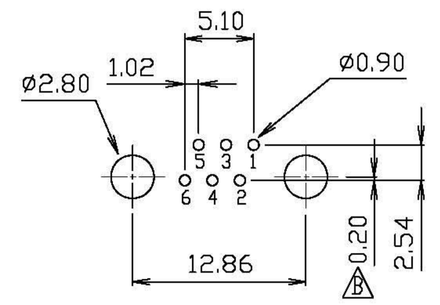
PCB LAYOUT Ref.
