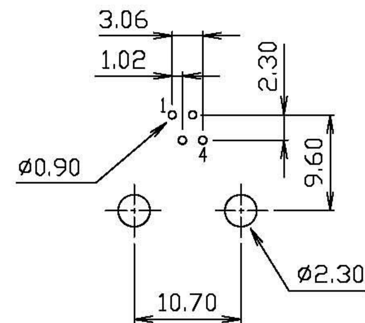
PCB LAYOUT Ref.
