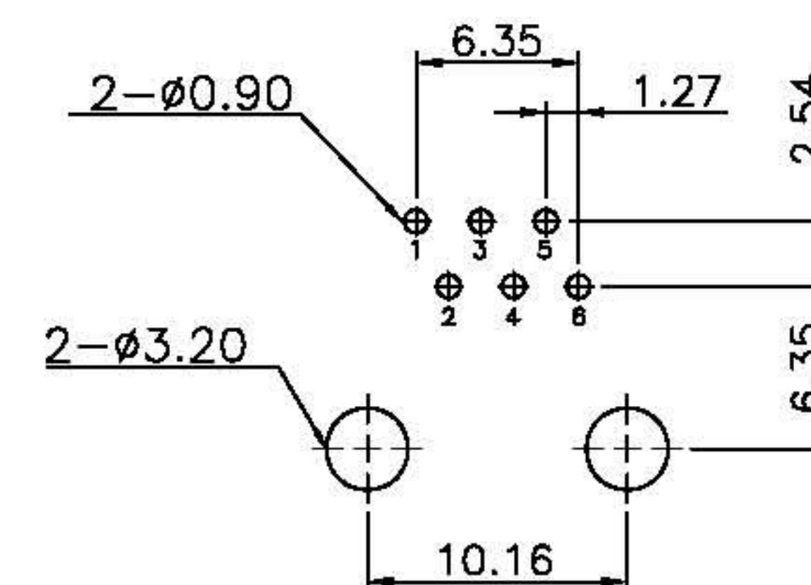
PCB LAYOUT (TOP VIEW) RECOMMENDED
