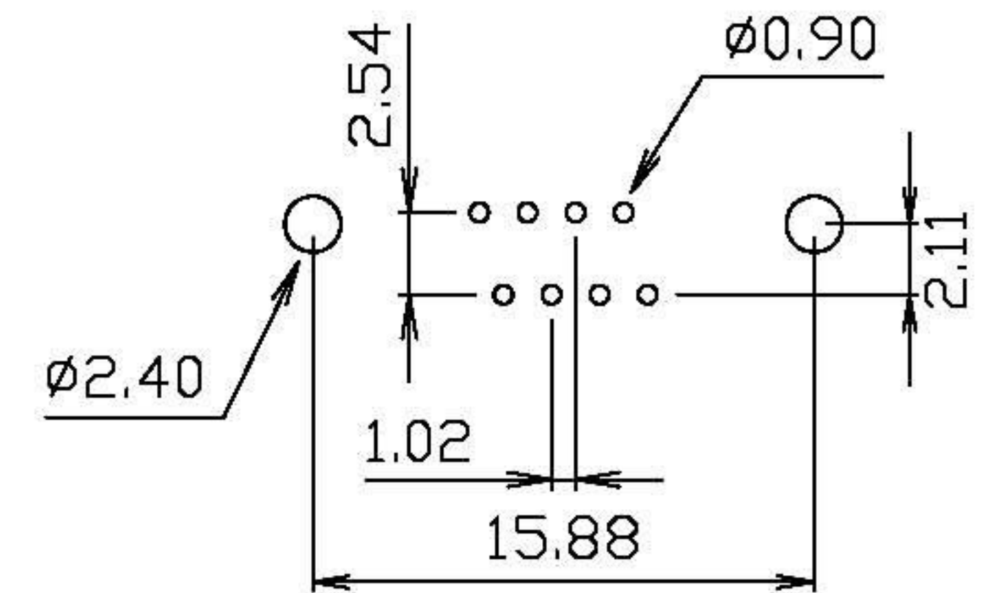
PC Board Layout
