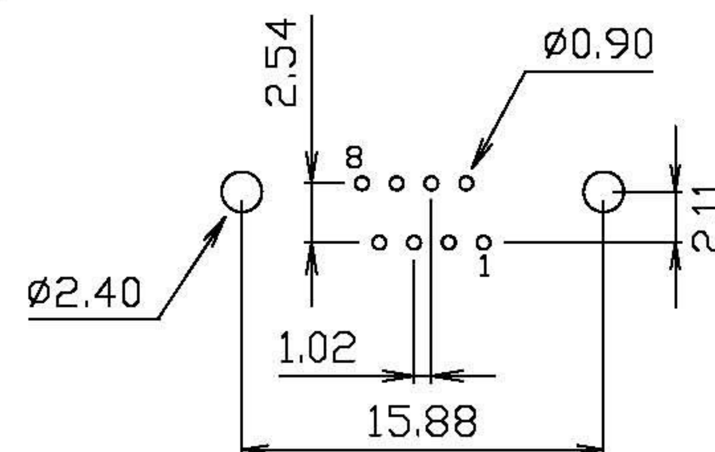
PC Board Layout Ref.
