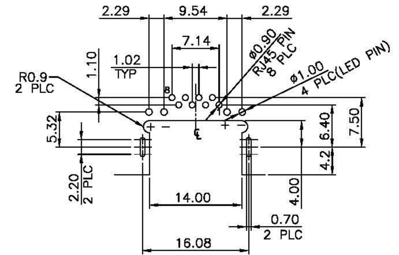
PCB LAYOUT Ref.
