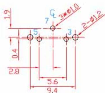
COMPONENT SIDE (PCB LAYOUT)
