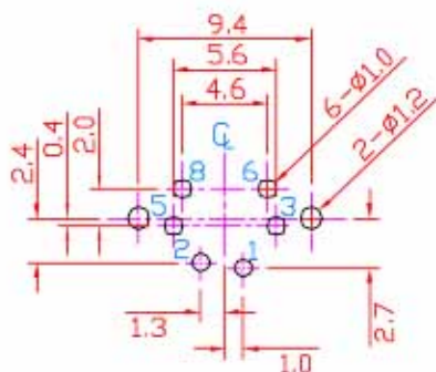
COMPONENT SIDE (PCB LAYOUT)
