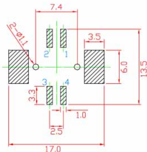
PCB LAYOUT (COMPONENT SIDE)
