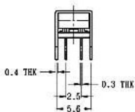
VIEW A SCALE 5:1
