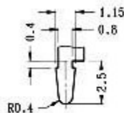
VIEW A SCALE 5:1
