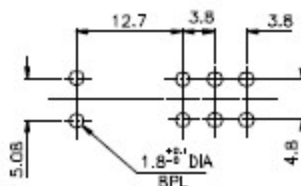
PRINTED CIRCUIT PANEL LAYOUT
